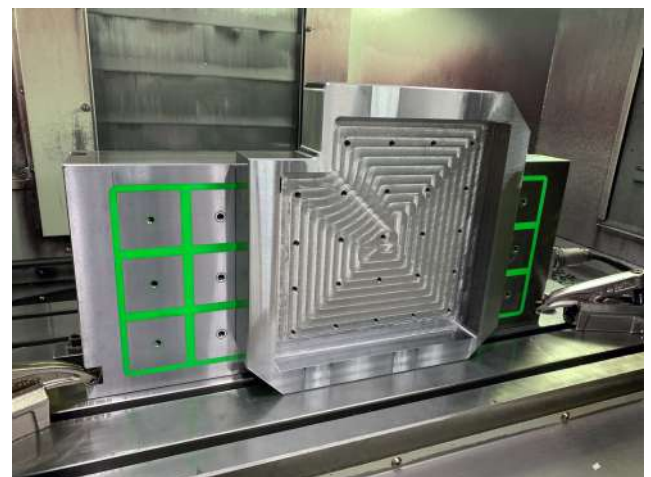
FXL Block expands the possibilities on 3 axis machines
