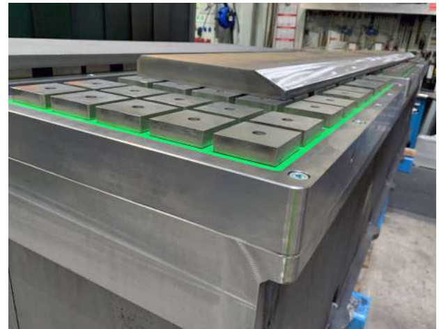
Weld edge preparation in large part manufacturing
