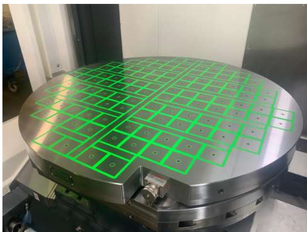
FXL-R magnetic clamping plate on a machining centre with rotary table D 1250 mm
